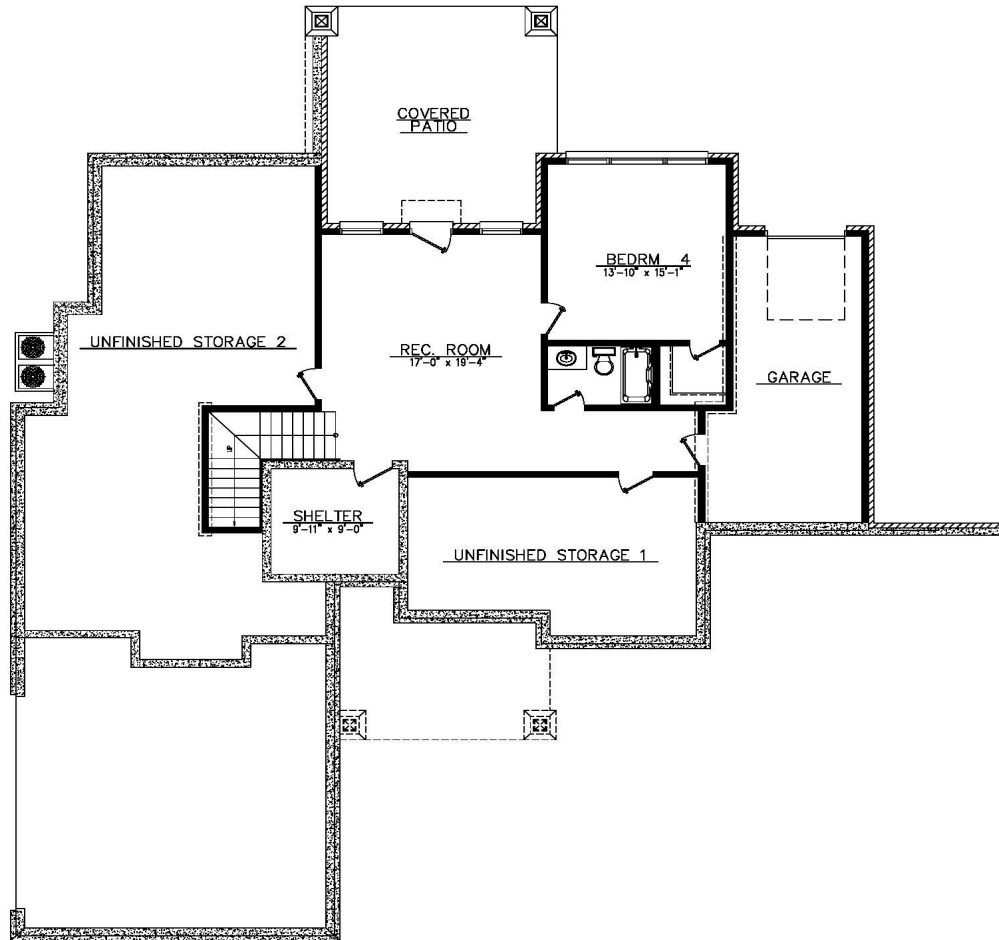
Basement Plan
